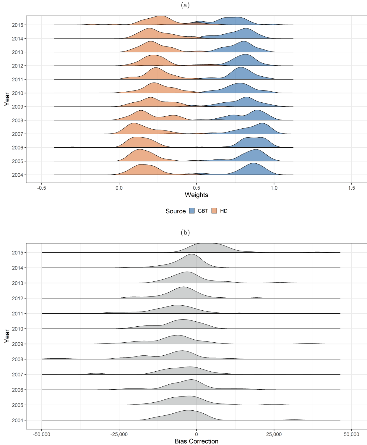
Figure A2: Forecast Combination Weights
